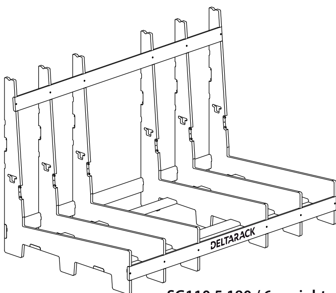
SG110.5.180 / 6 uprights
