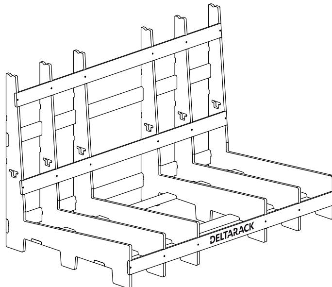
SG110.7.180 / 6 uprights
