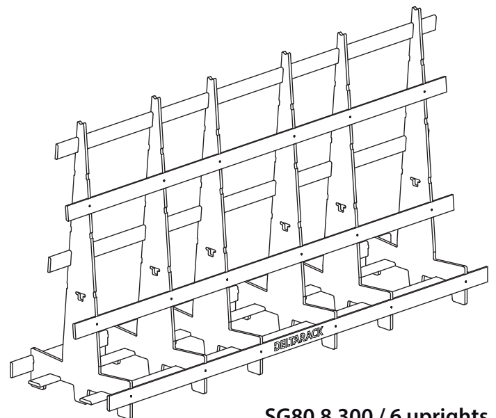
SG80.8.300 / 6 uprights
