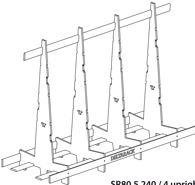
SR80.5.240 / 4 uprights
