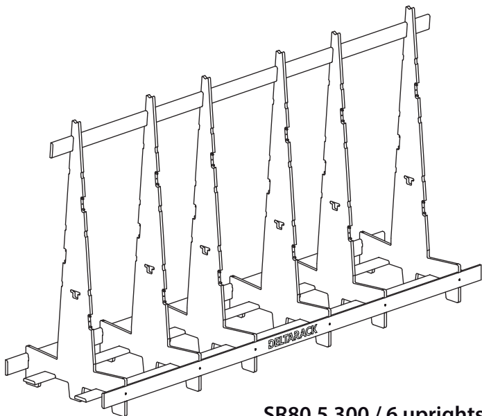
SR80.5.300 / 6 uprights
