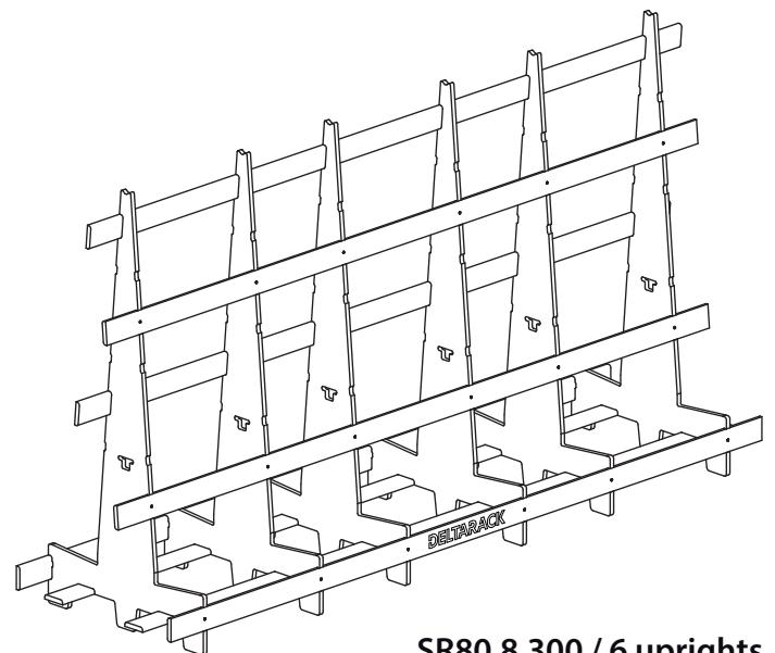
SR80.8.300 / 6 uprights
